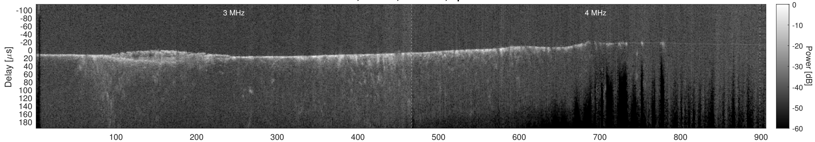
Orbit 11668, Cluttergram
