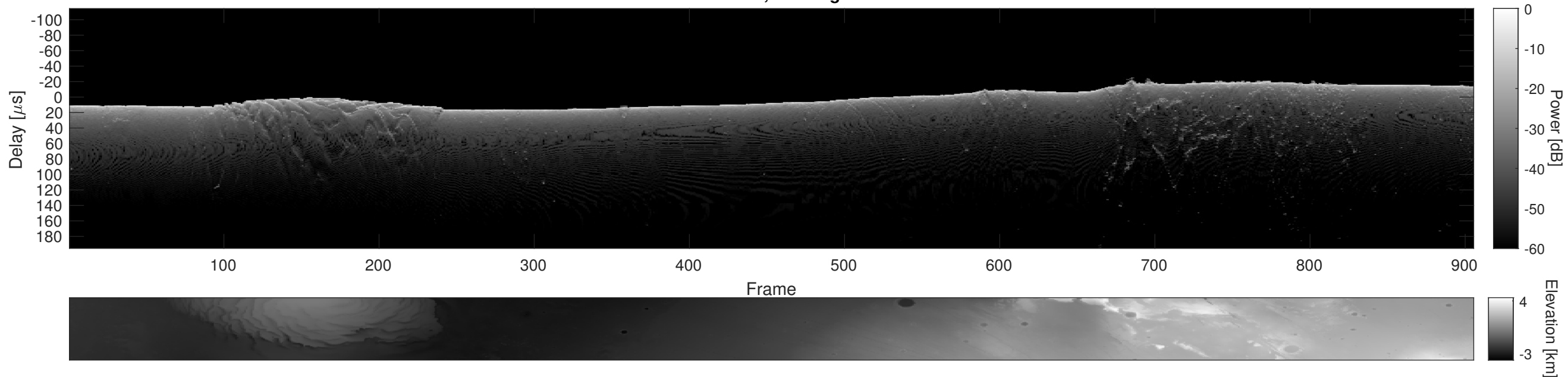
Orbit 11668, Cluttergram
