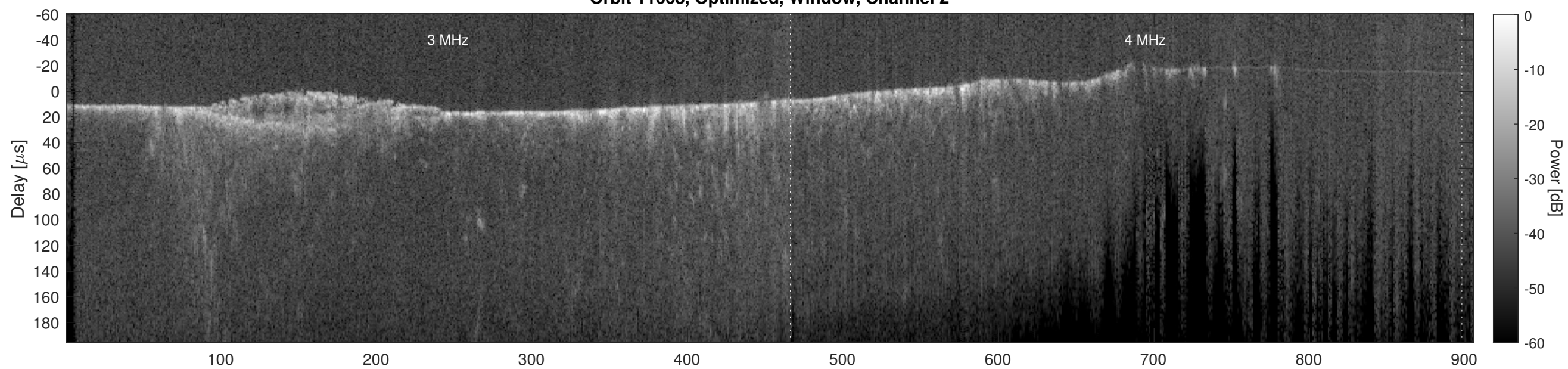
Orbit 11668, Cluttergram
