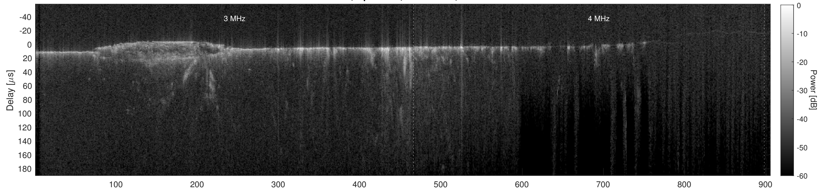
Orbit 11670, Cluttergram
