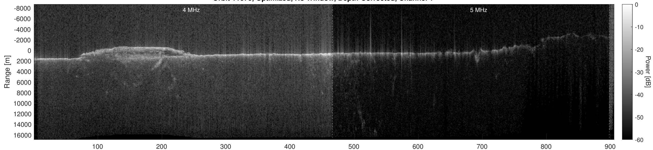
Orbit 11670, Optimized, No Window, Depth-Corrected, Channel 2
