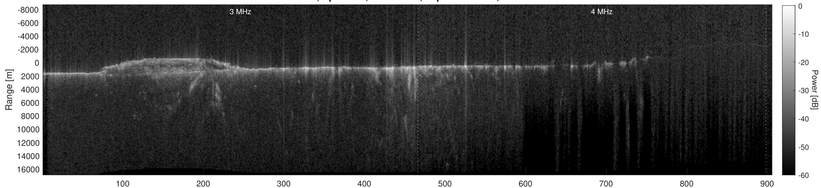
Orbit 11670, Depth-Corrected Cluttergram
