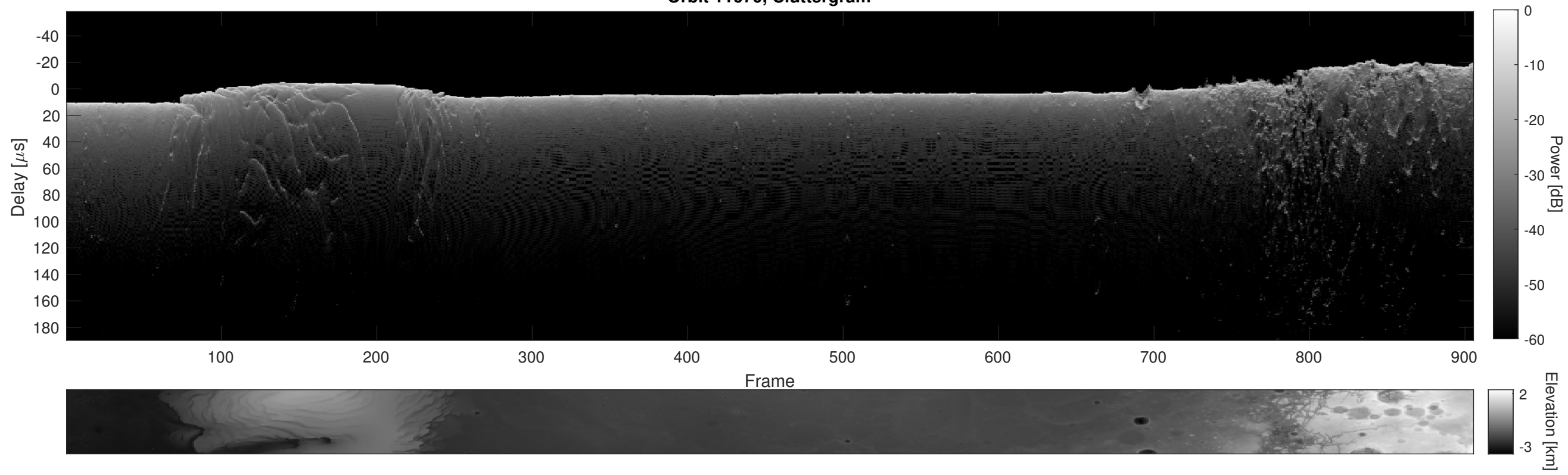
Orbit 11670, Cluttergram
