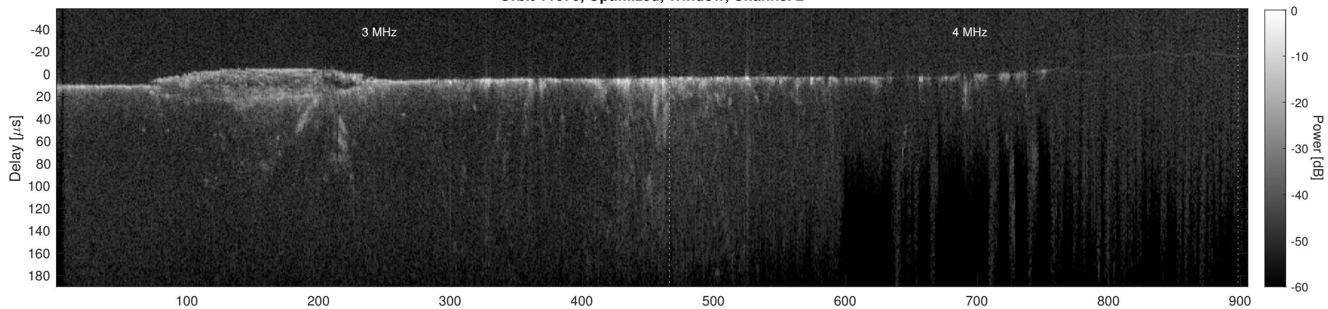
Orbit 11670, Cluttergram
