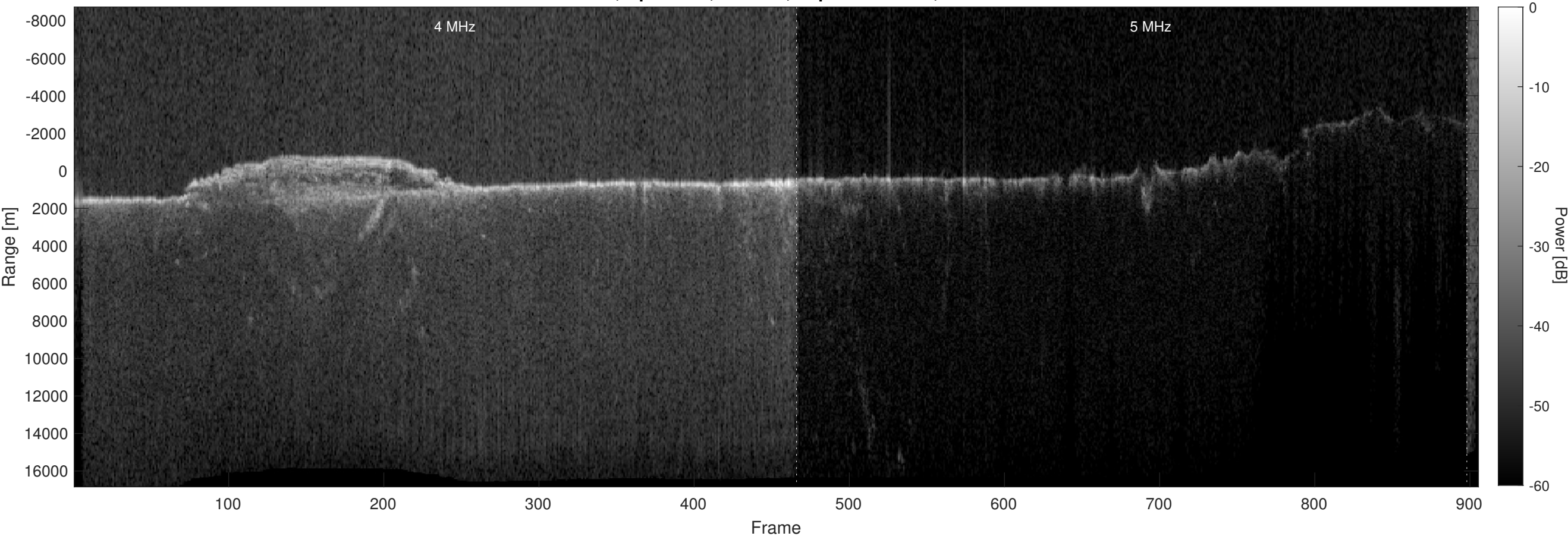
Orbit 11670, Optimized, Window, Depth-Corrected, Channel 2
