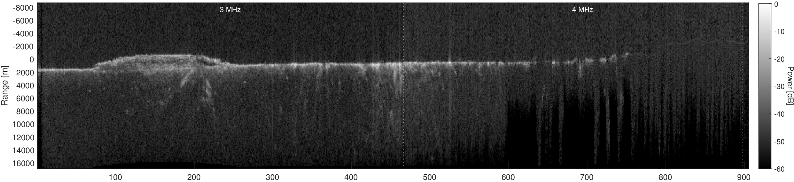
Orbit 11670, Depth-Corrected Cluttergram
