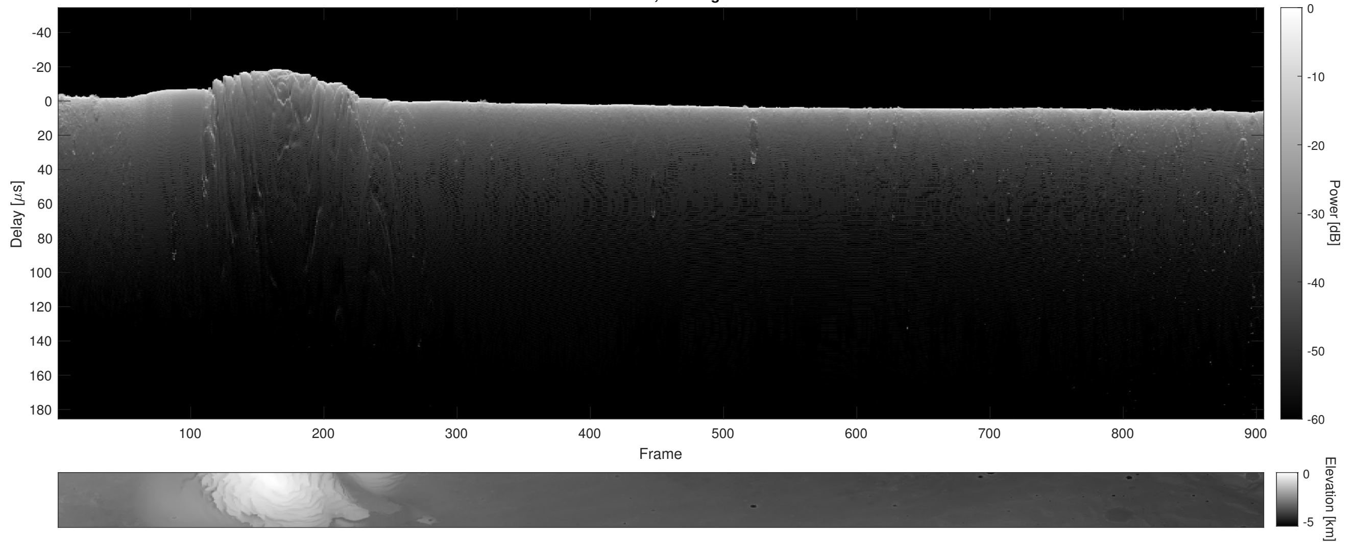
Orbit 11671, Cluttergram
