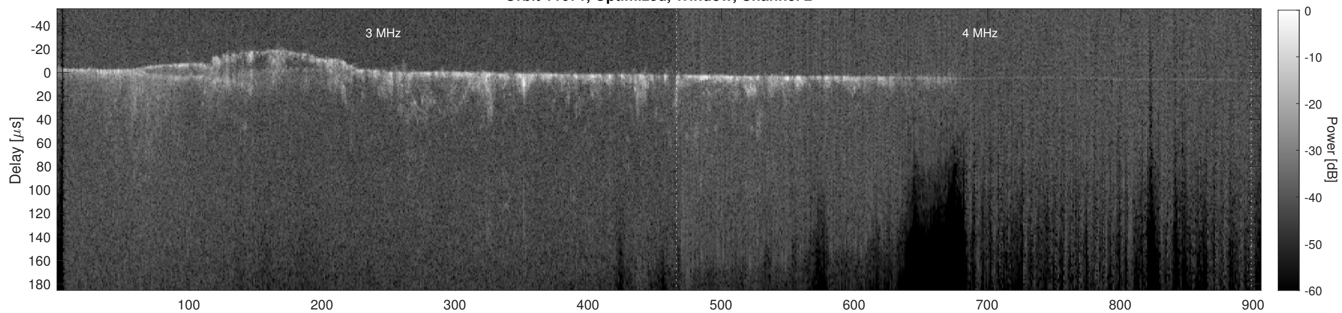
Orbit 11671, Cluttergram
