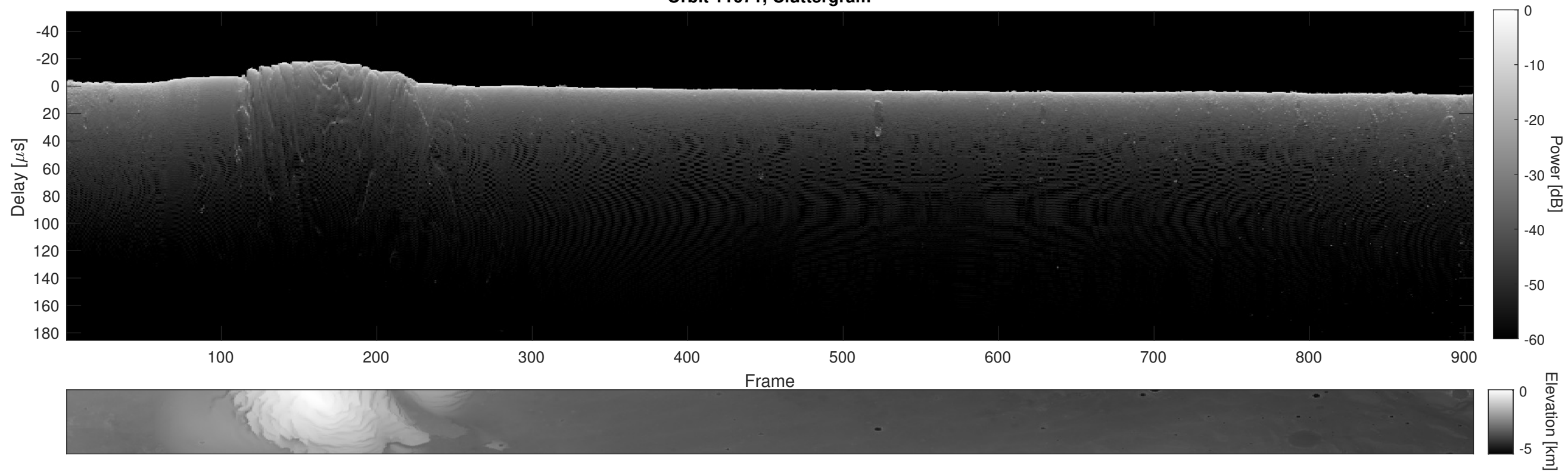
Orbit 11671, Cluttergram
