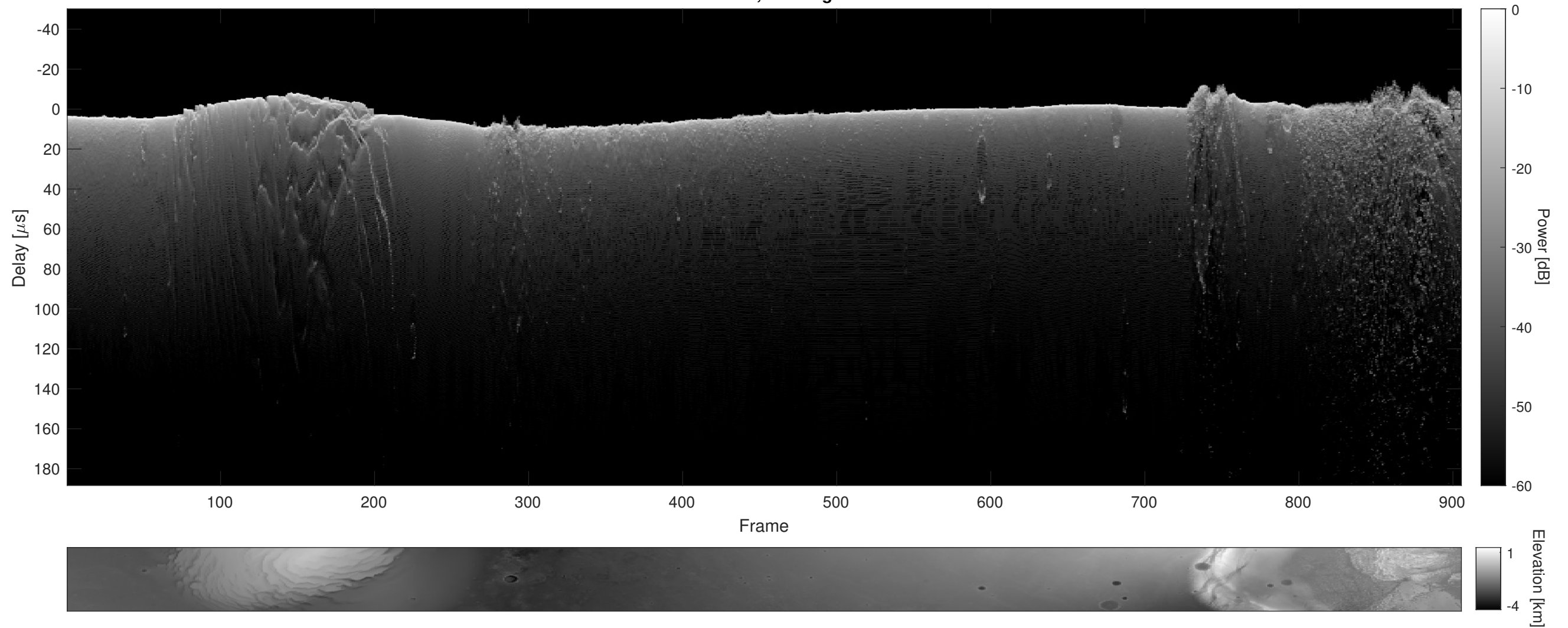
Orbit 11672, Cluttergram
