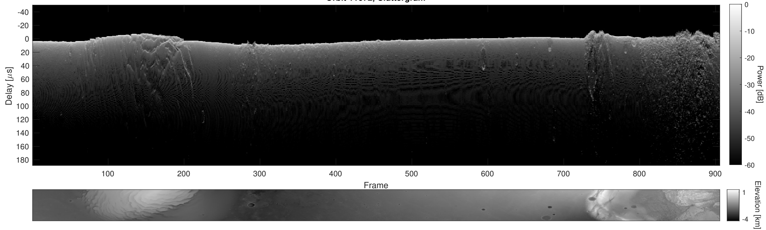
Orbit 11672, Cluttergram
