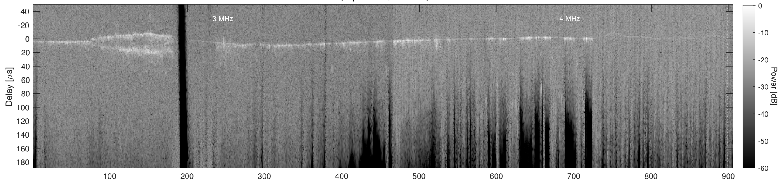
Orbit 11672, Cluttergram
