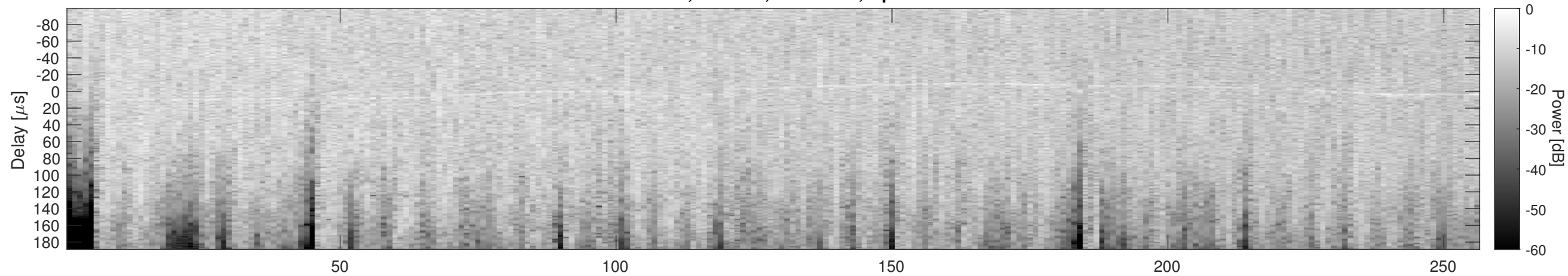
Orbit 11673, Cluttergram
