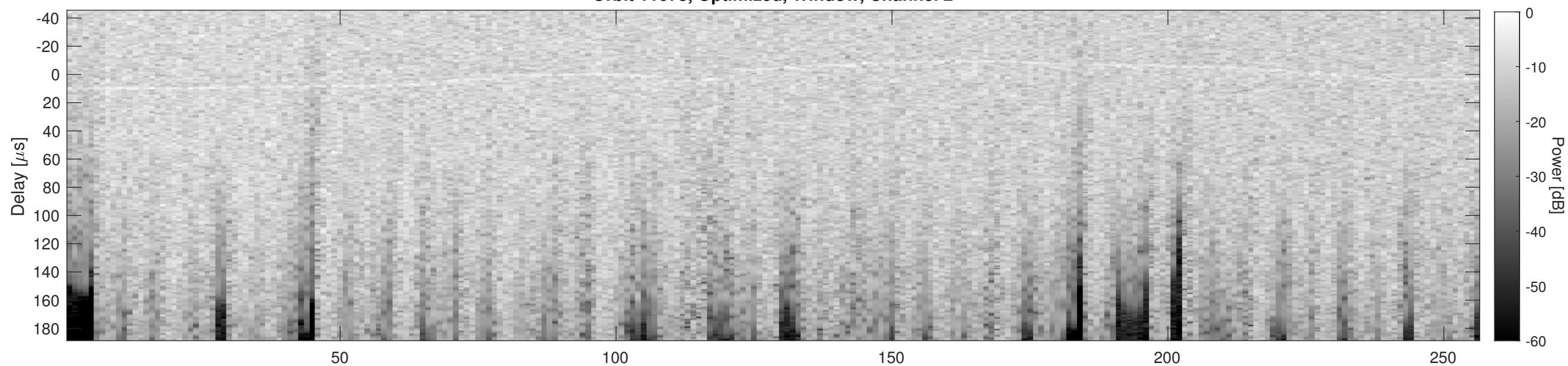
Orbit 11673, Cluttergram
