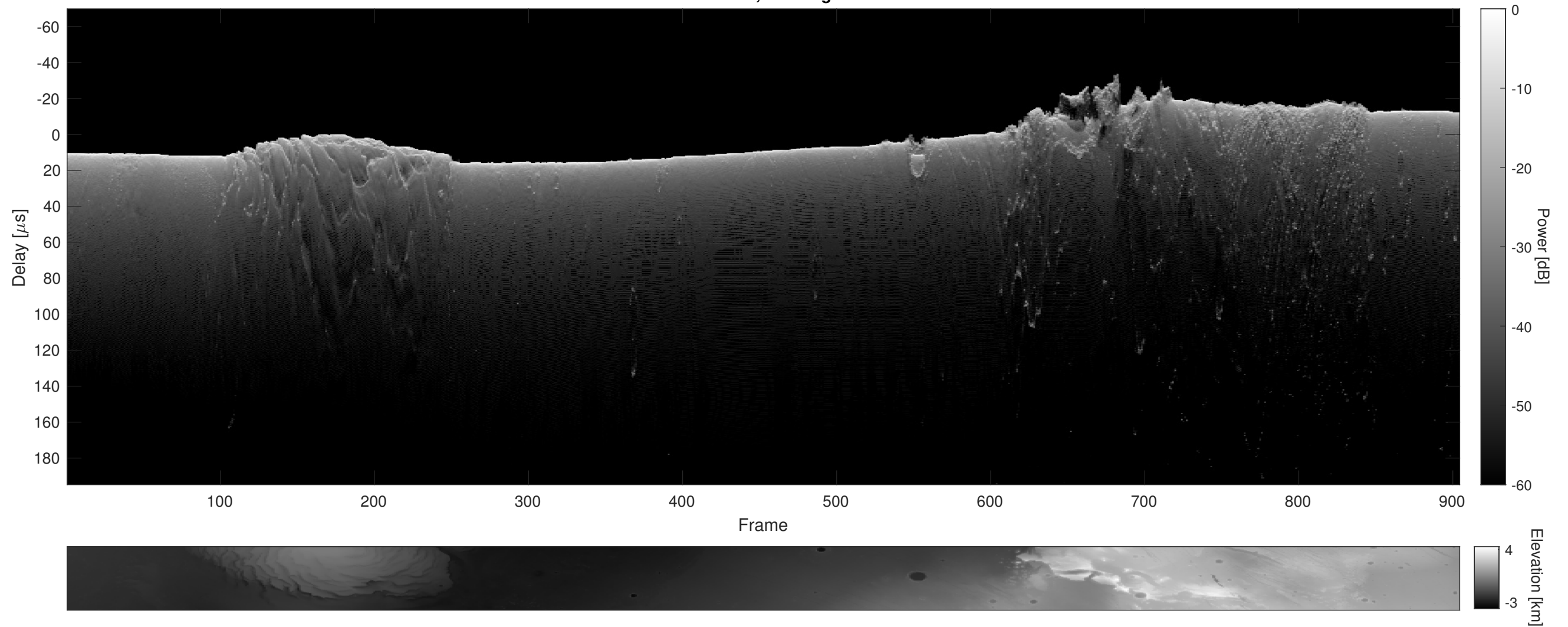
Orbit 11675, Cluttergram
