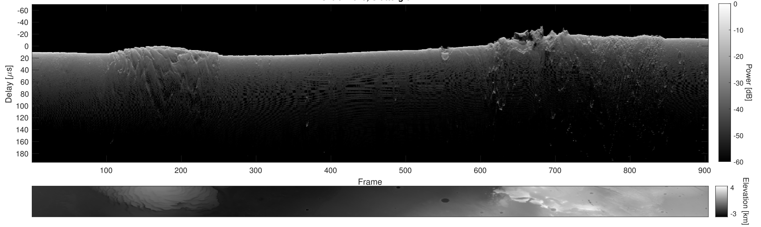
Orbit 11675, Cluttergram
