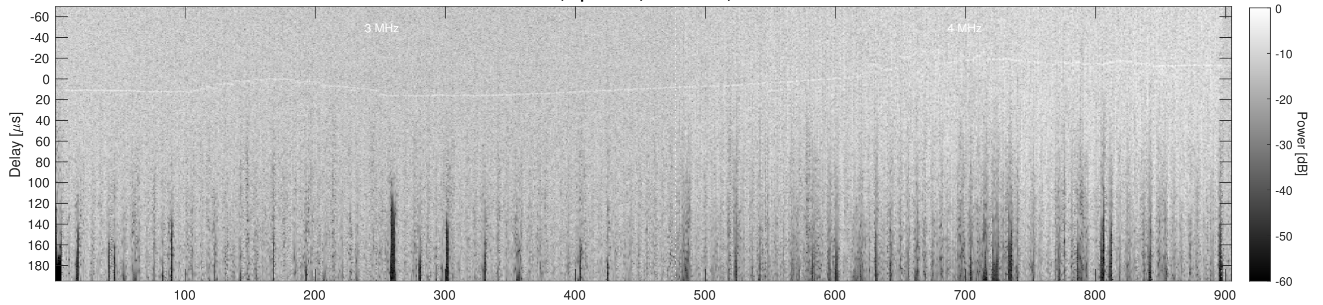
Orbit 11675, Cluttergram
