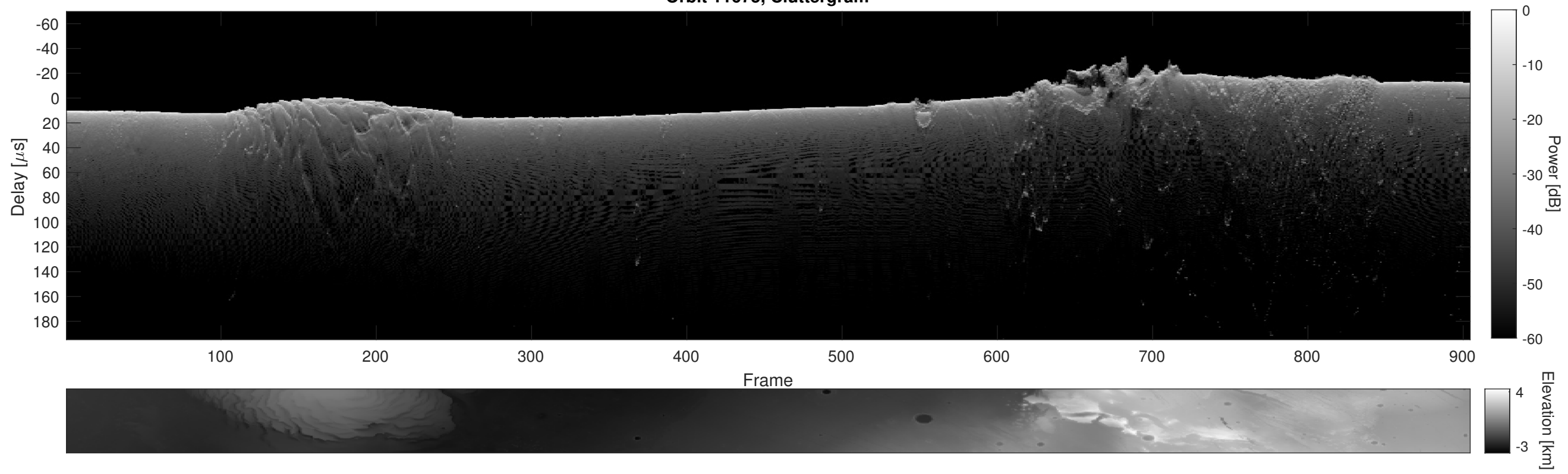
Orbit 11675, Cluttergram
