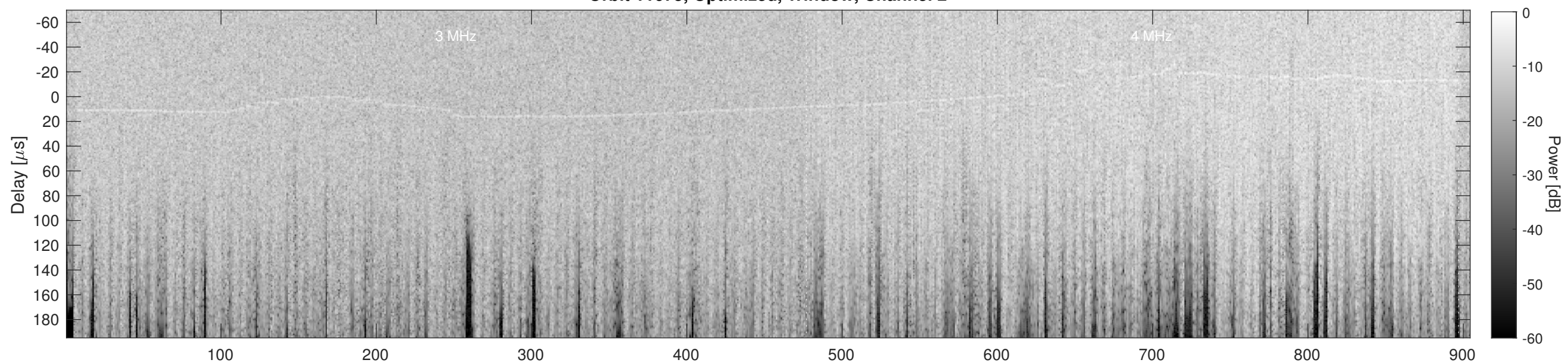
Orbit 11675, Cluttergram
