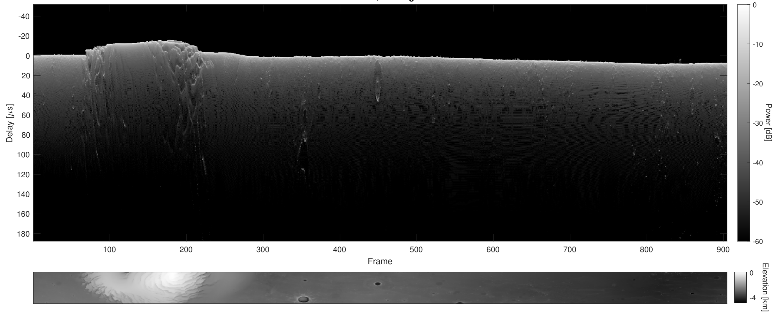
Orbit 11683, Cluttergram
