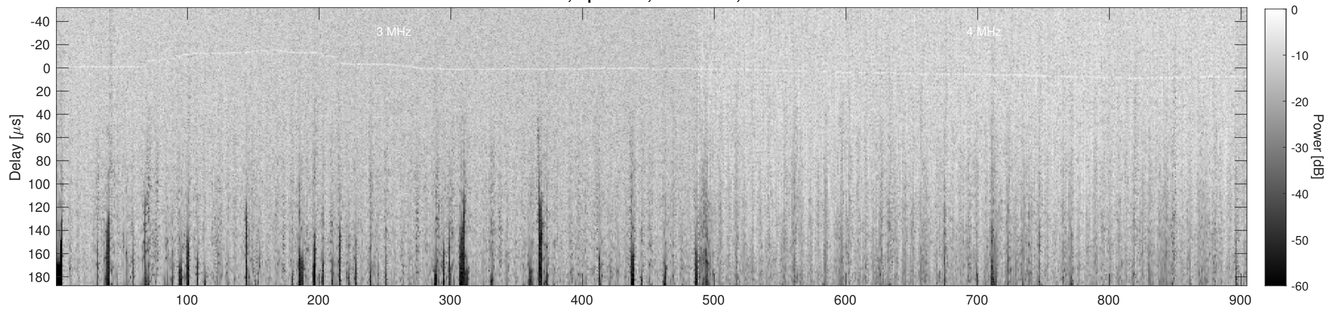
Orbit 11683, Cluttergram
