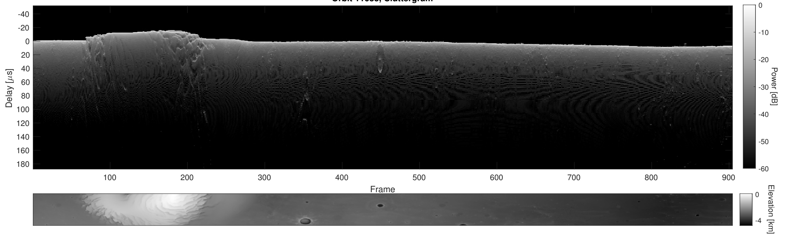
Orbit 11683, Cluttergram
