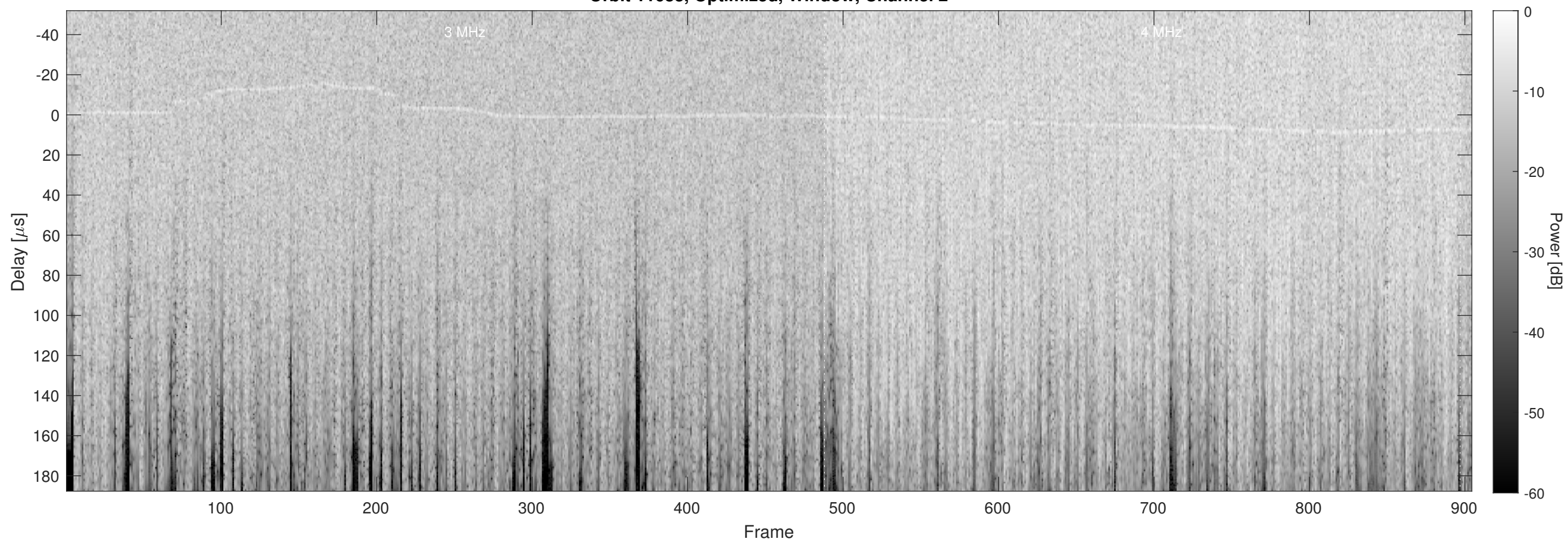
Orbit 11683, Optimized, Window, Channel 2
