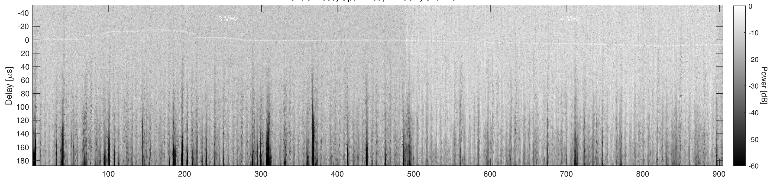
Orbit 11683, Cluttergram
