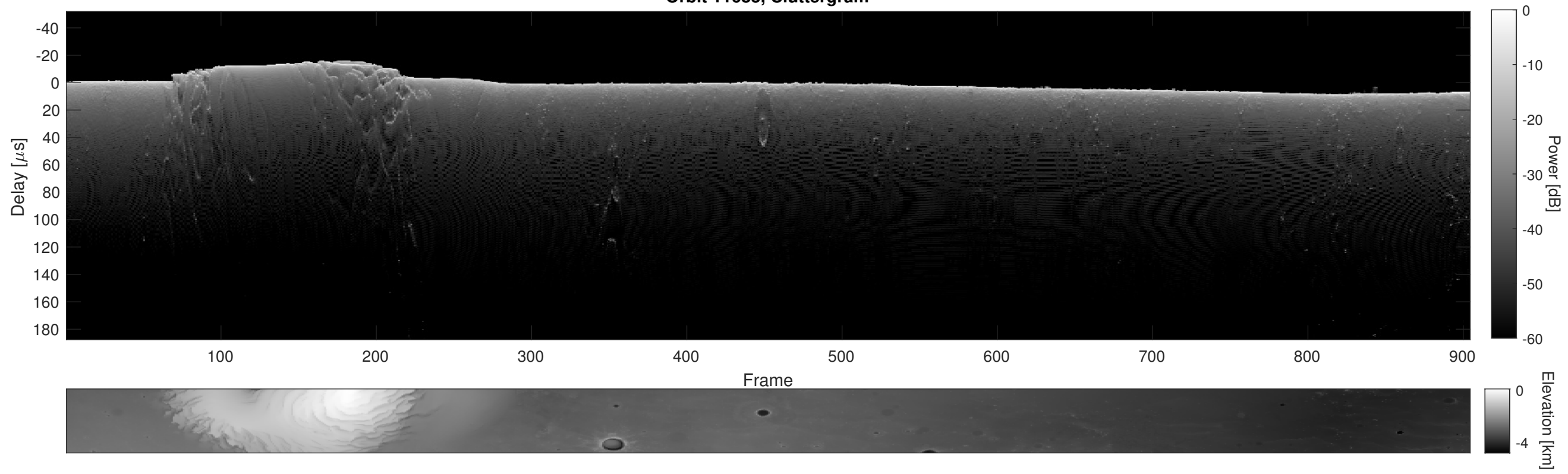
Orbit 11683, Cluttergram
