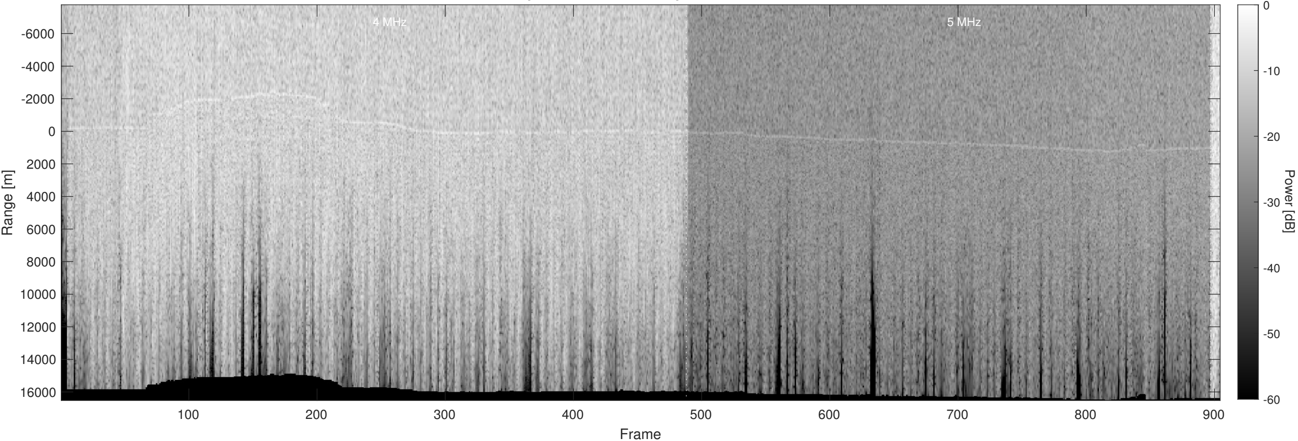
Orbit 11683, Optimized, Window, Depth-Corrected, Channel 2
