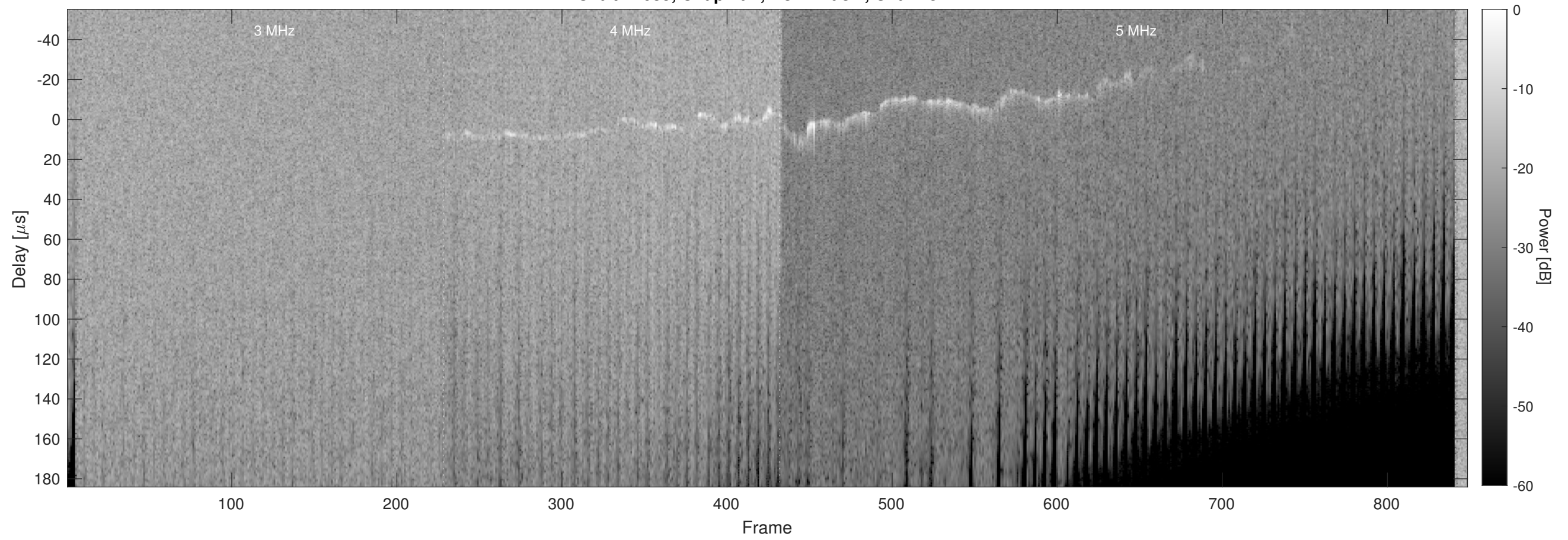
Orbit 11685, Chapman, No Window, Channel 2
