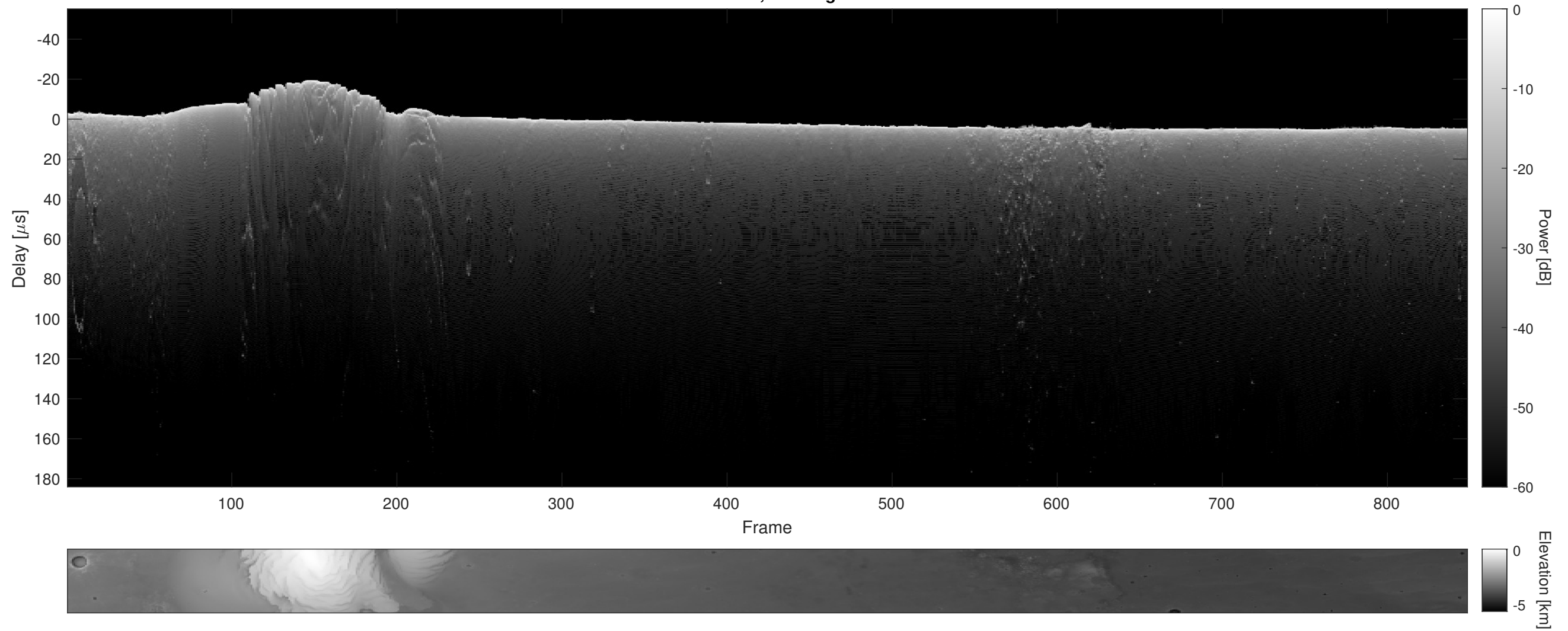
Orbit 11685, Cluttergram
