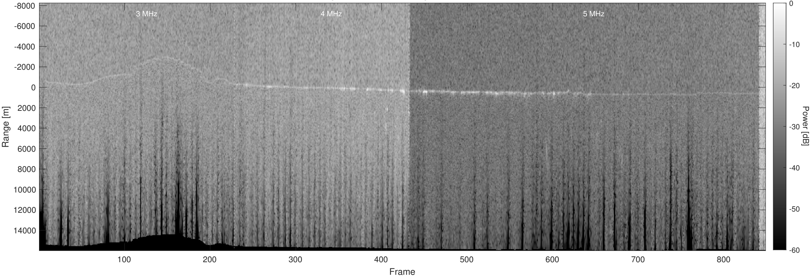
Orbit 11685, Optimized, Window, Depth-Corrected, Channel 2
