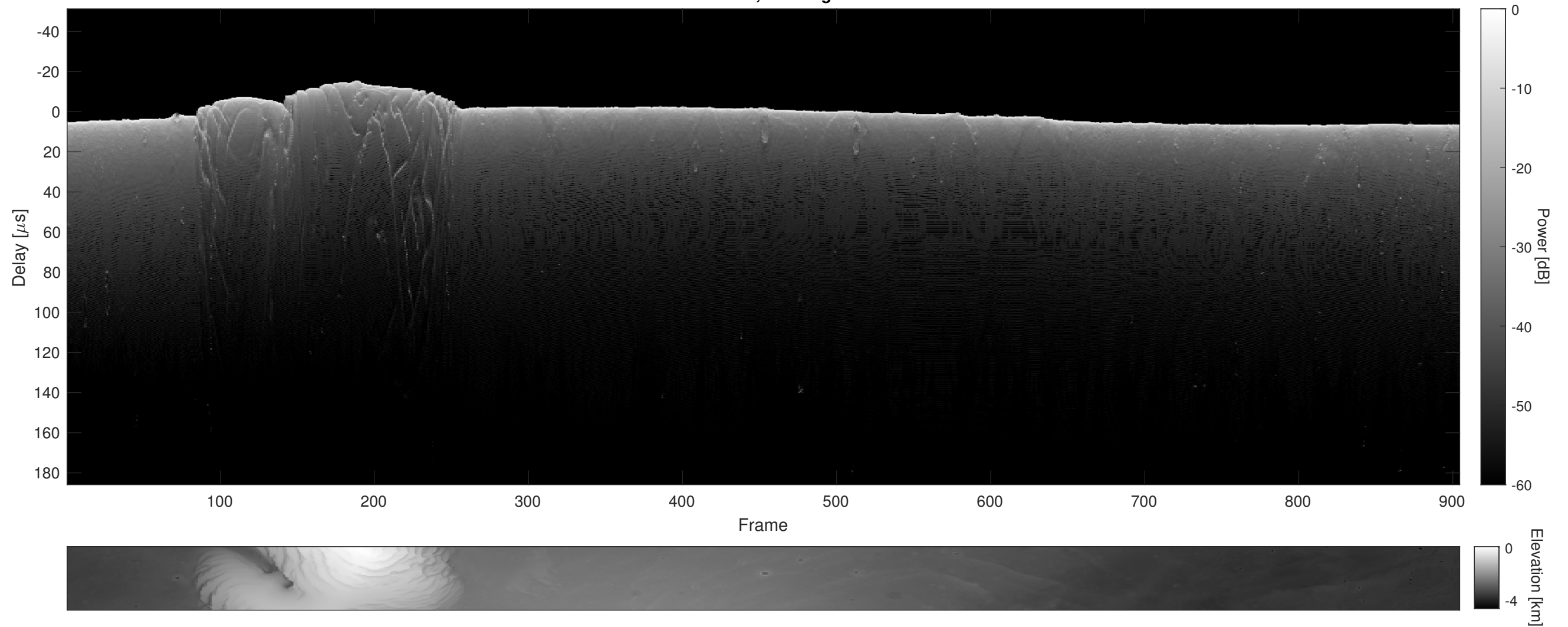
Orbit 11687, Cluttergram
