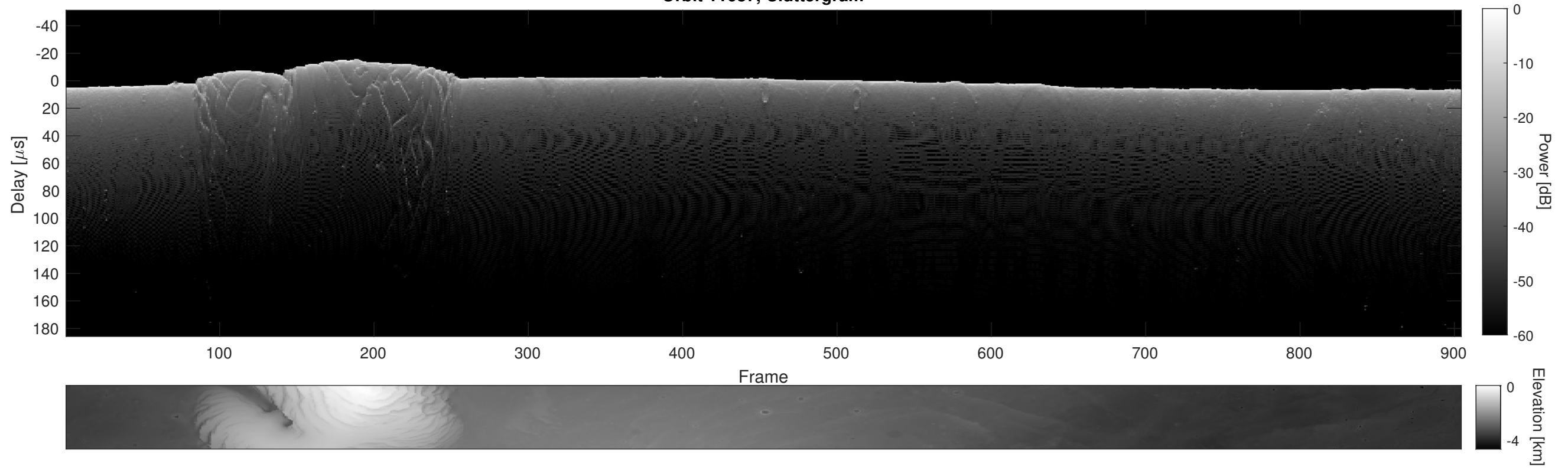
Orbit 11687, Cluttergram
