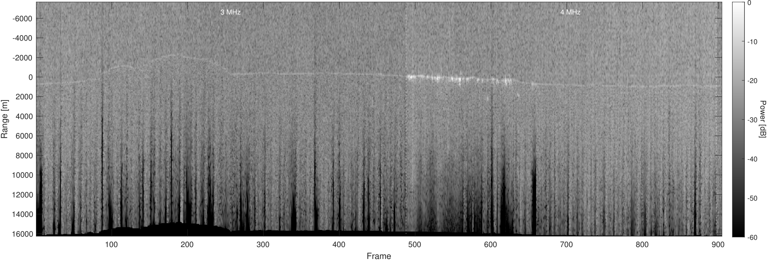
Orbit 11687, Optimized, Window, Depth-Corrected, Channel 2
