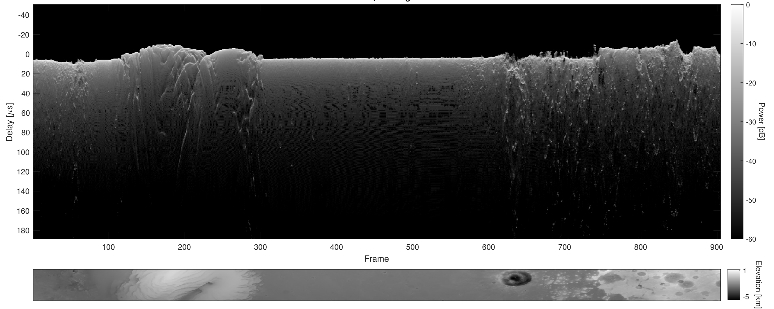
Orbit 11688, Cluttergram
