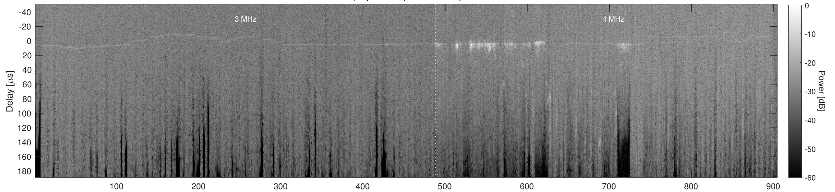
Orbit 11688, Cluttergram
