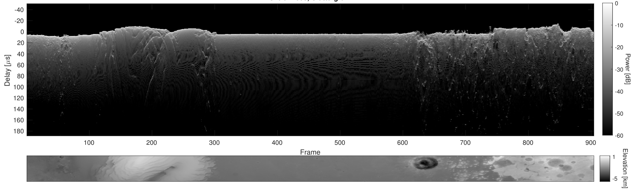
Orbit 11688, Cluttergram
