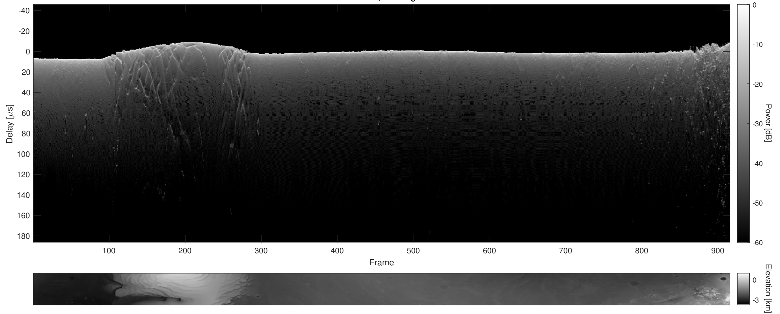
Orbit 11691, Cluttergram
