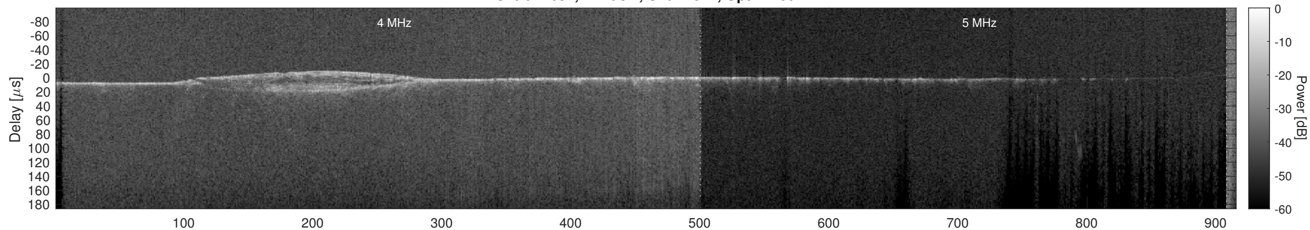
Orbit 11691, Cluttergram
