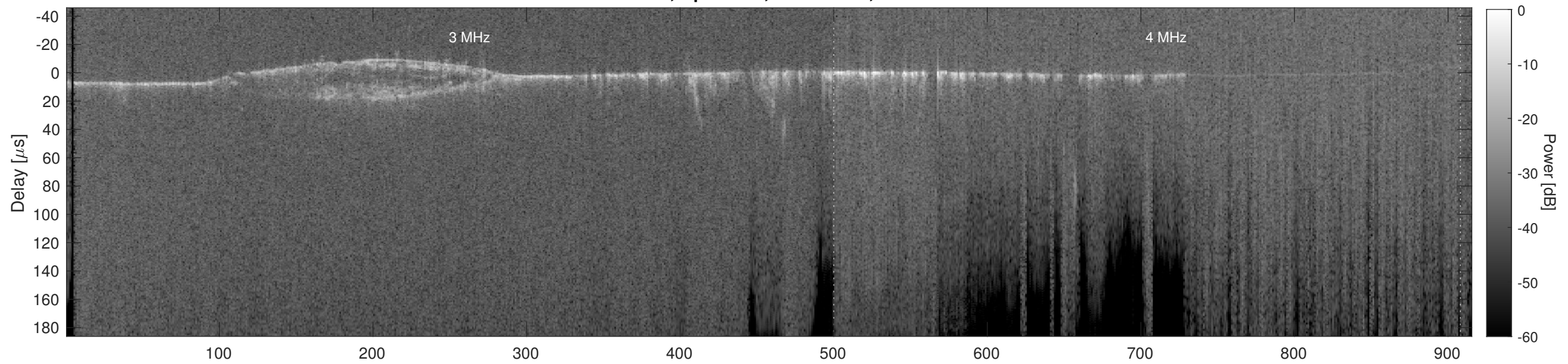
Orbit 11691, Cluttergram
