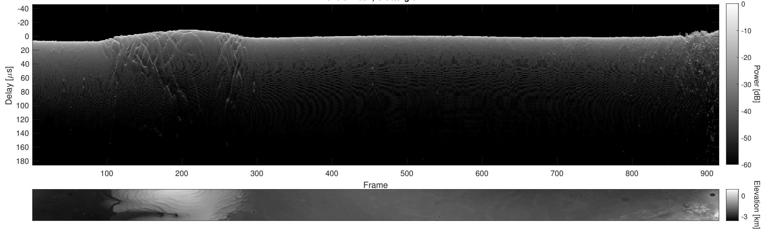
Orbit 11691, Cluttergram
