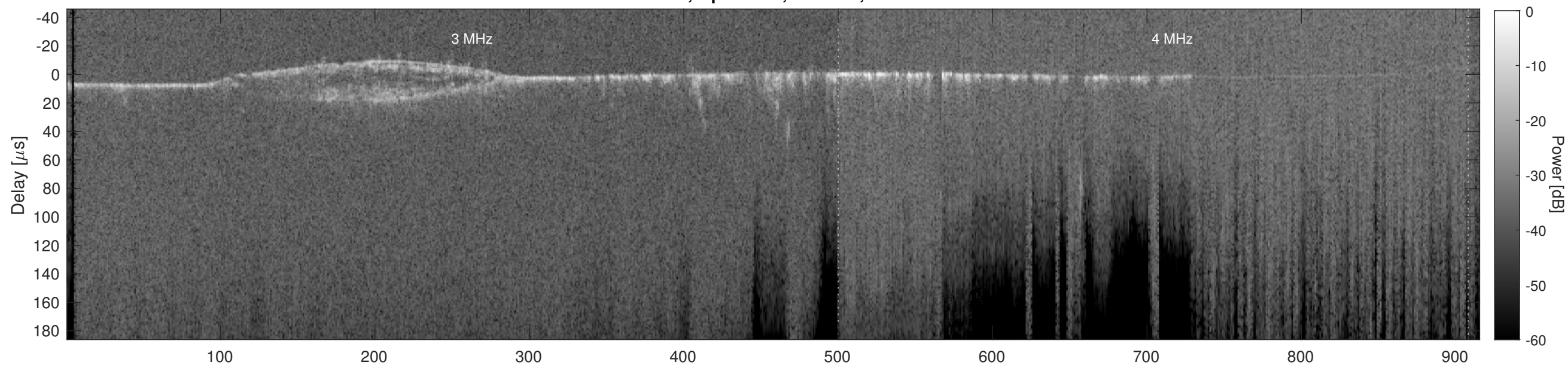
Orbit 11691, Cluttergram
