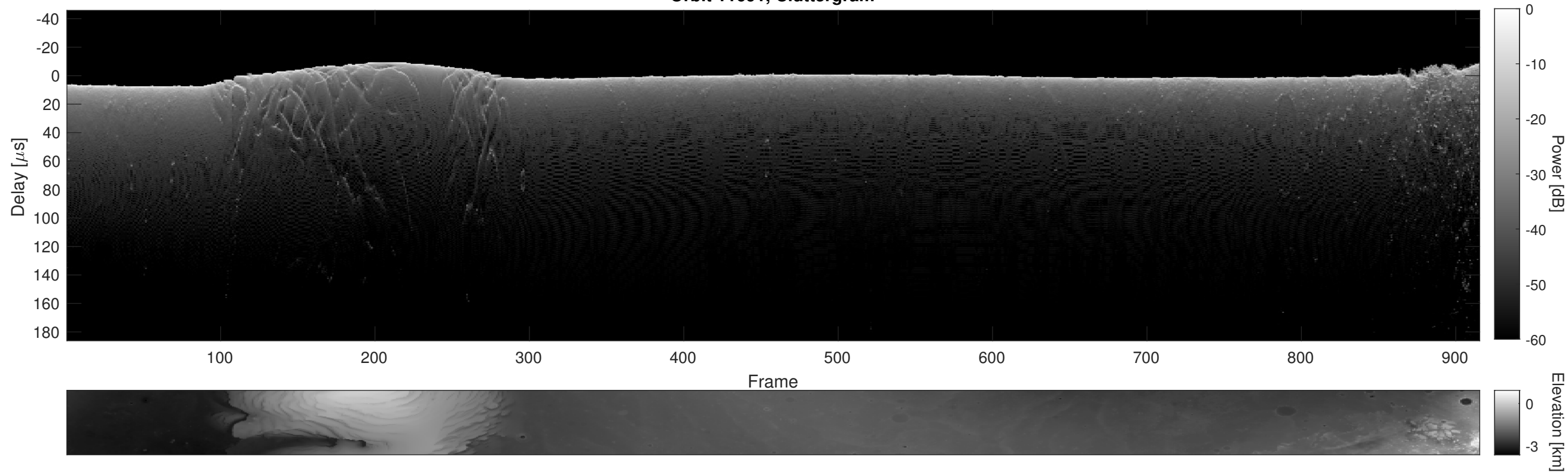
Orbit 11691, Cluttergram
