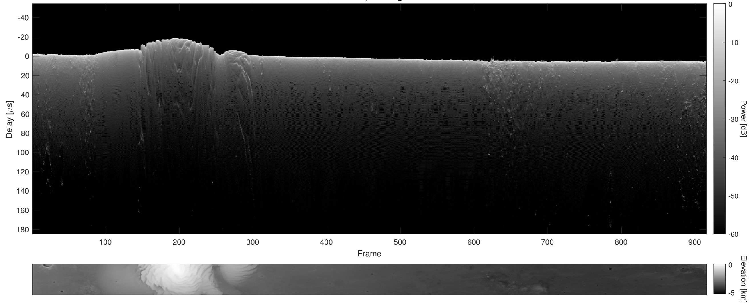
Orbit 11692, Cluttergram
