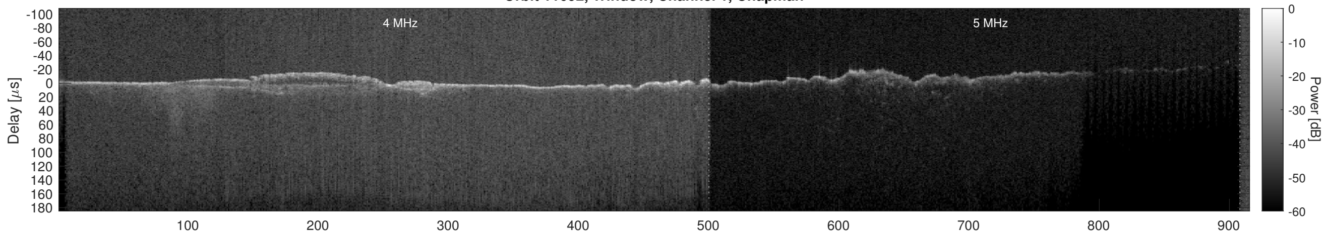
Orbit 11692, Window, Channel 1, Optimized
