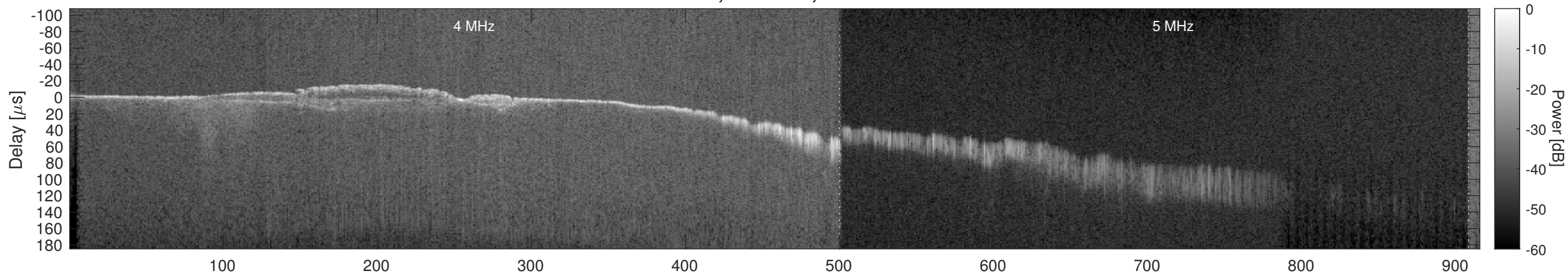
Orbit 11692, Window, Channel 1, Chapman
