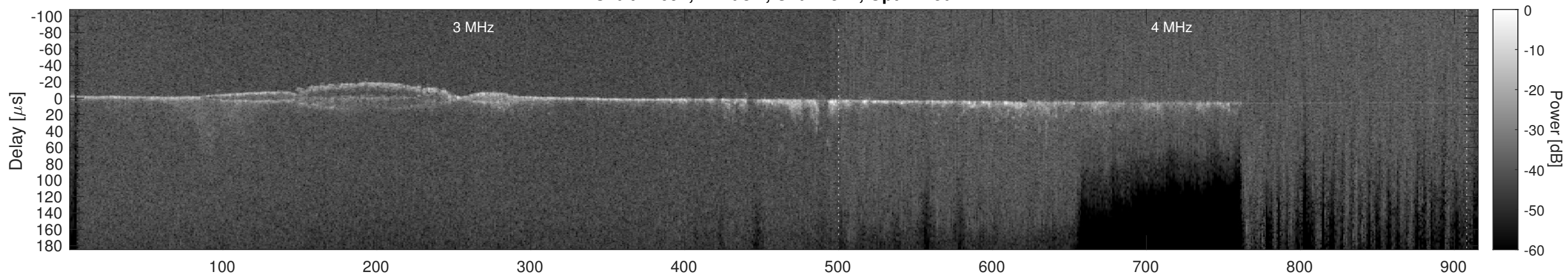
Orbit 11692, Cluttergram
