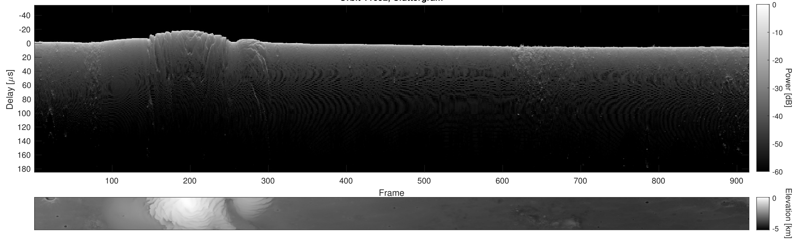
Orbit 11692, Cluttergram
