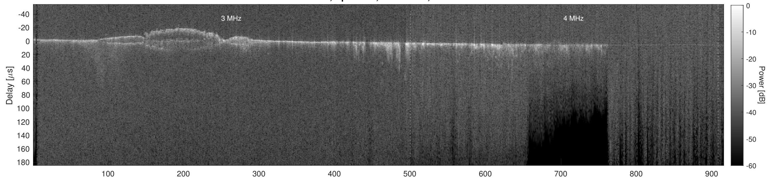
Orbit 11692, Cluttergram
