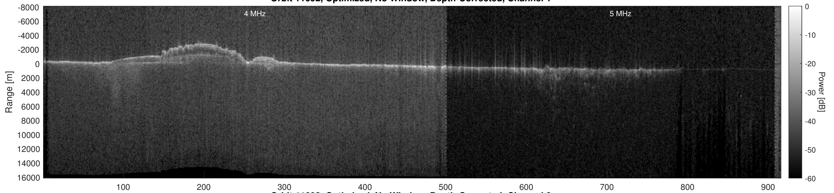
Orbit 11692, Optimized, No Window, Depth-Corrected, Channel 2
