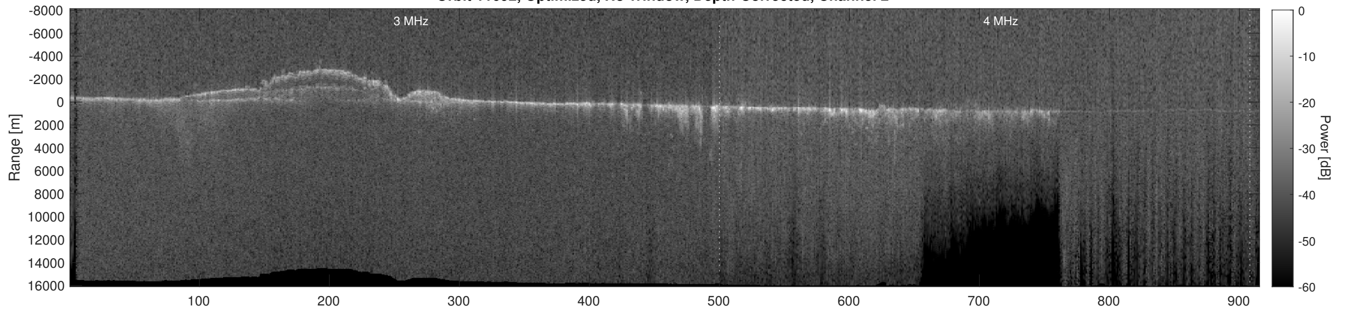
Orbit 11692, Depth-Corrected Cluttergram
