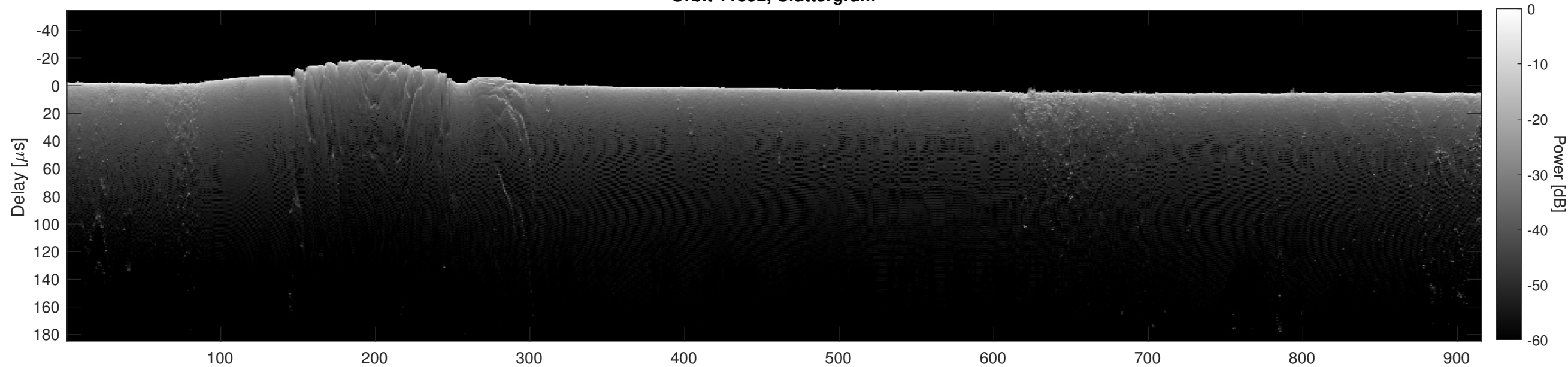
Orbit 11692, Cluttergram
