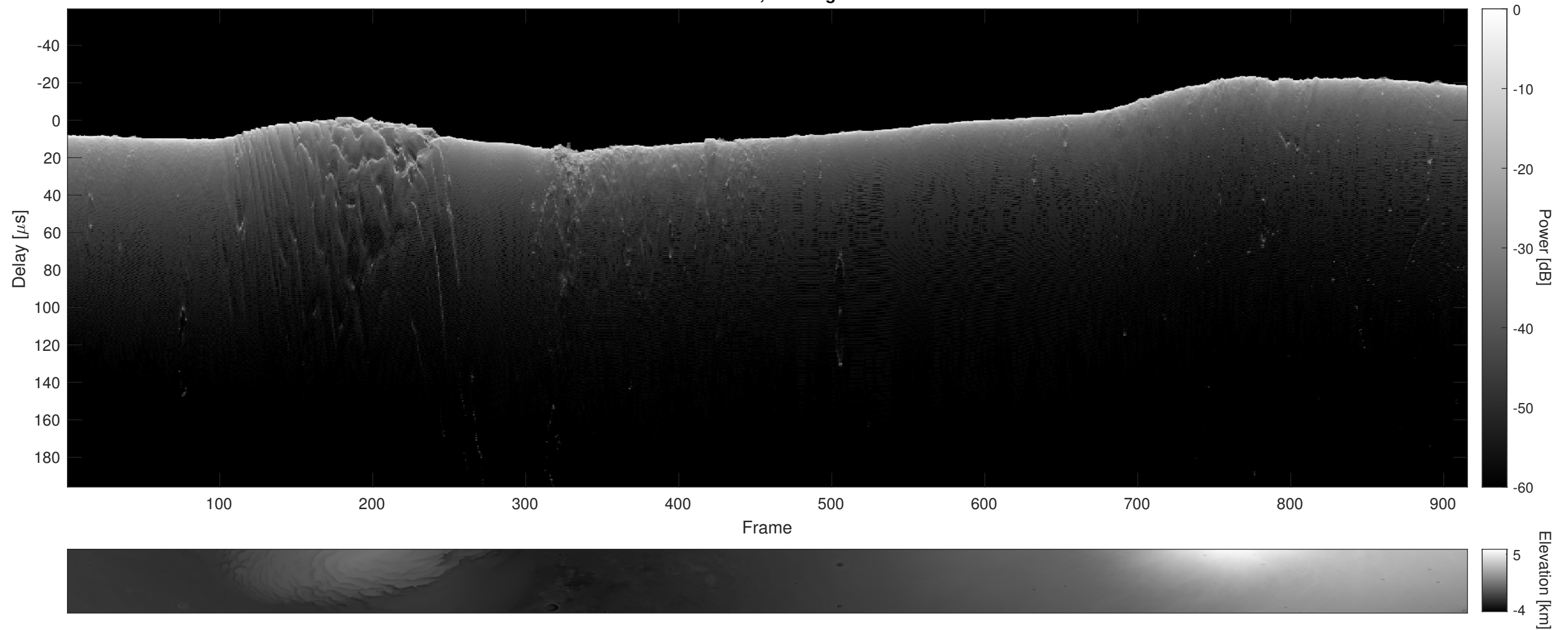
Orbit 11693, Cluttergram
