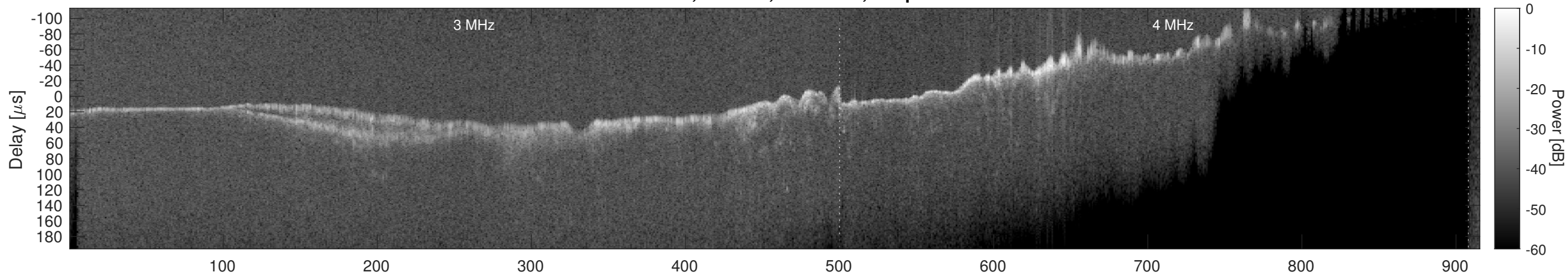
Orbit 11693, Window, Channel 2, Optimized
