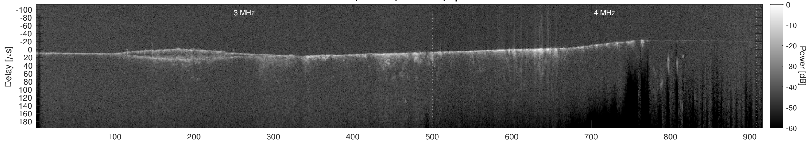
Orbit 11693, Cluttergram
