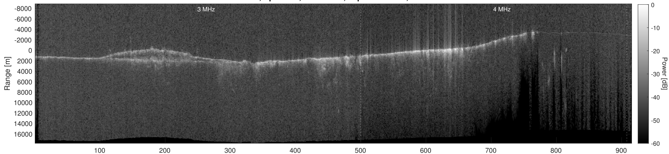
Orbit 11693, Depth-Corrected Cluttergram
