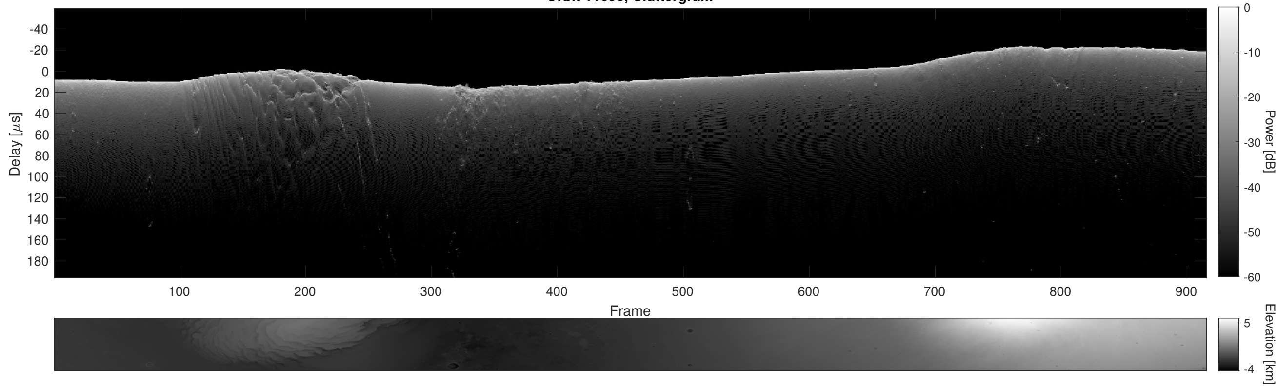
Orbit 11693, Cluttergram
