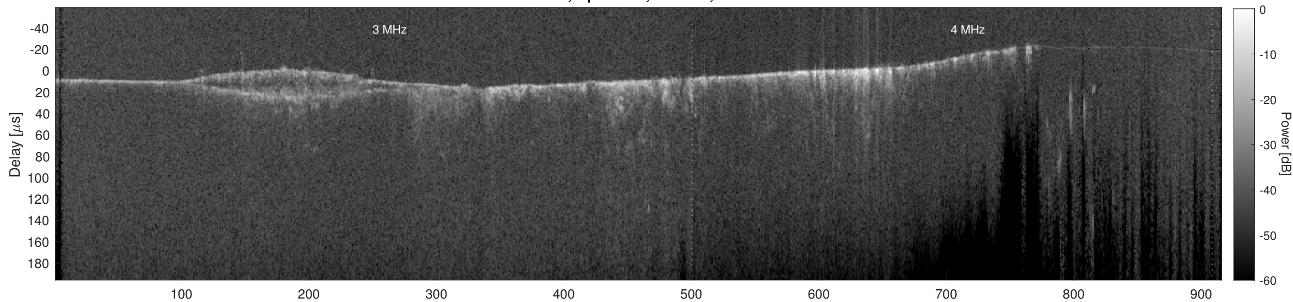
Orbit 11693, Cluttergram
