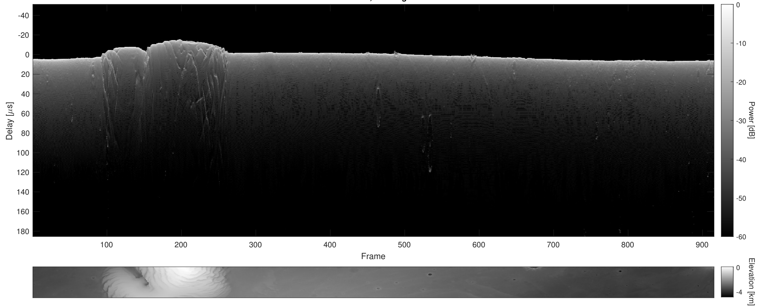
Orbit 11694, Cluttergram
