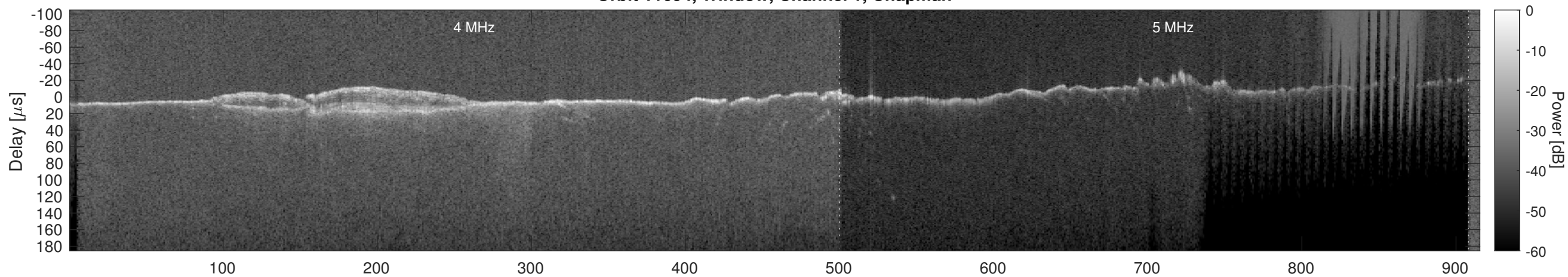
Orbit 11694, Window, Channel 1, Optimized
