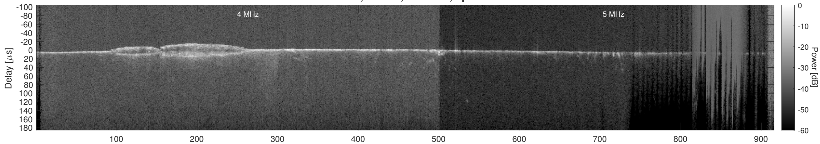
Orbit 11694, Cluttergram
