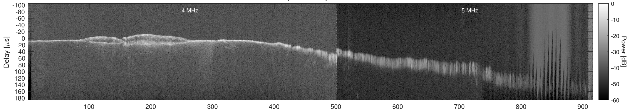
Orbit 11694, Window, Channel 1, Chapman
