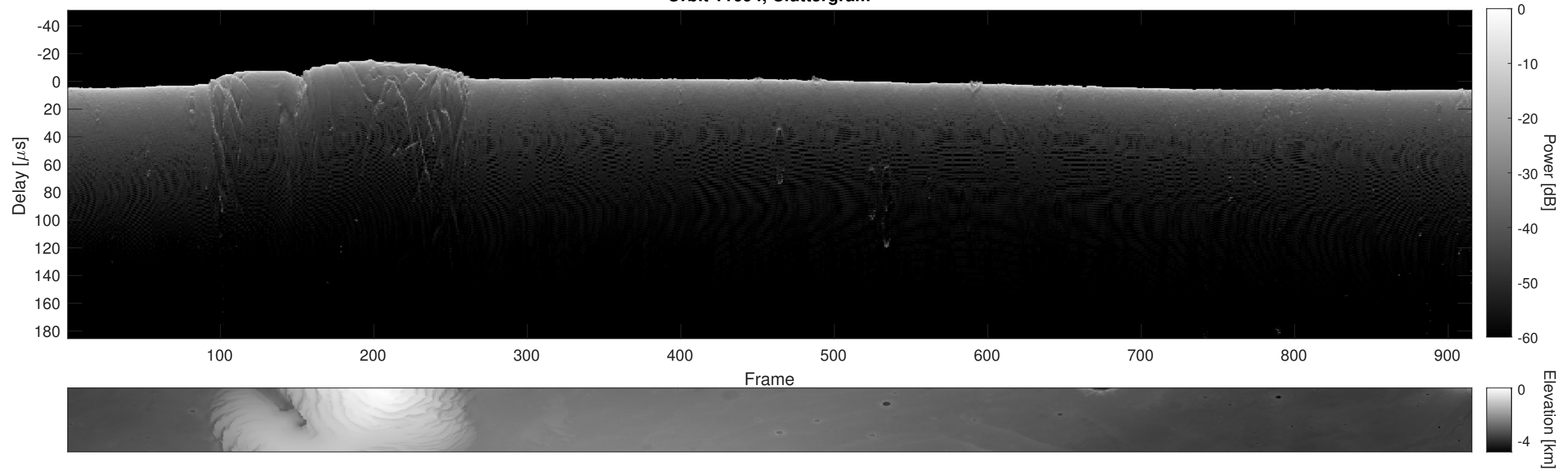
Orbit 11694, Cluttergram
