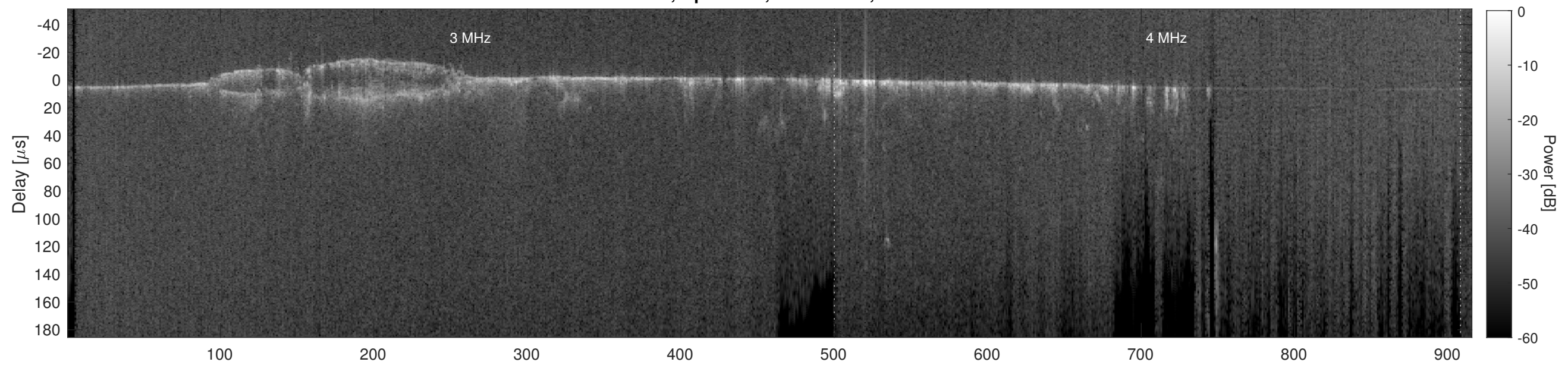
Orbit 11694, Cluttergram
