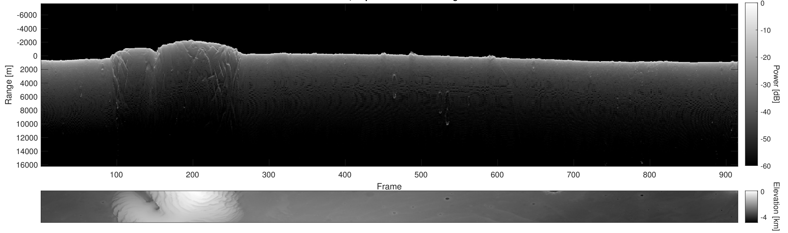
Orbit 11694, Depth-Corrected Cluttergram
