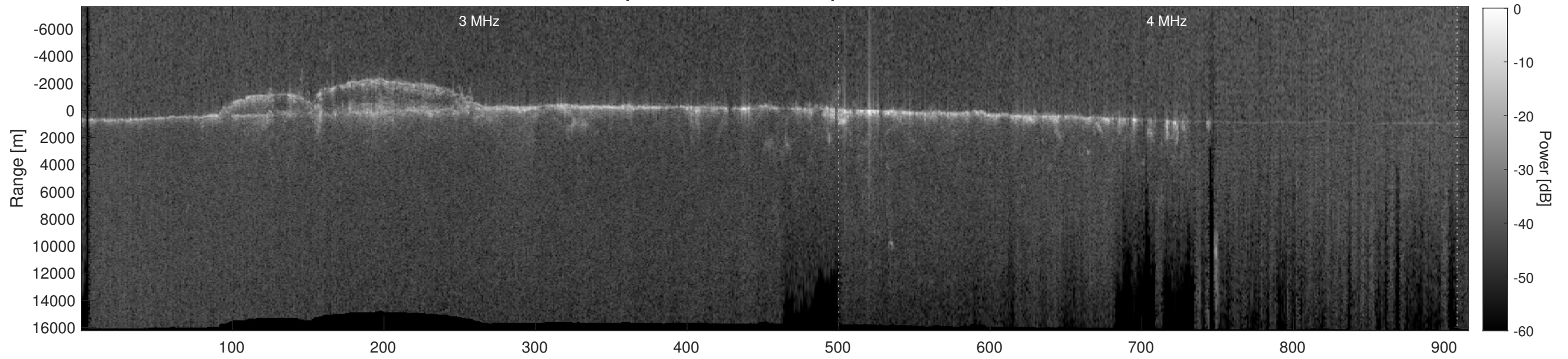
Orbit 11694, Depth-Corrected Cluttergram
