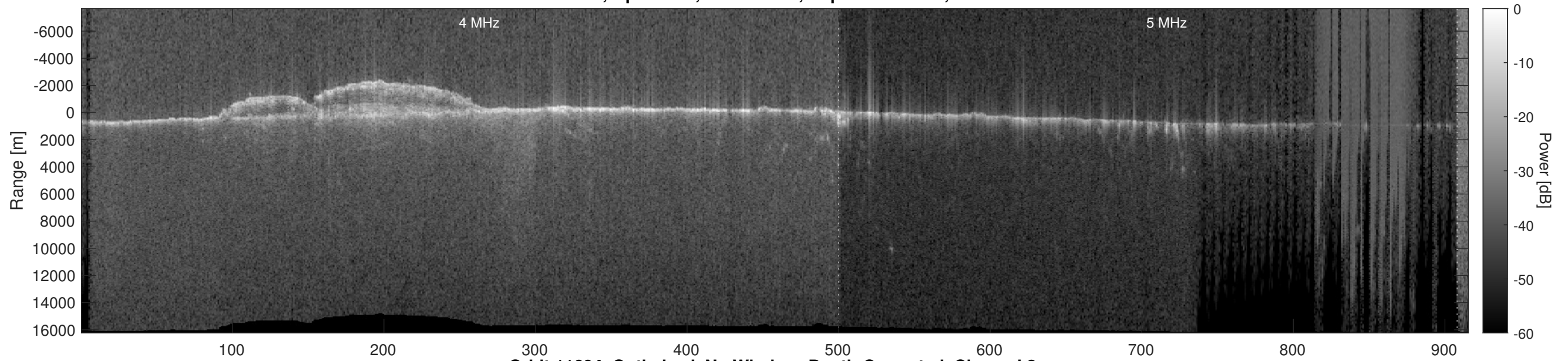
Orbit 11694, Optimized, No Window, Depth-Corrected, Channel 2
