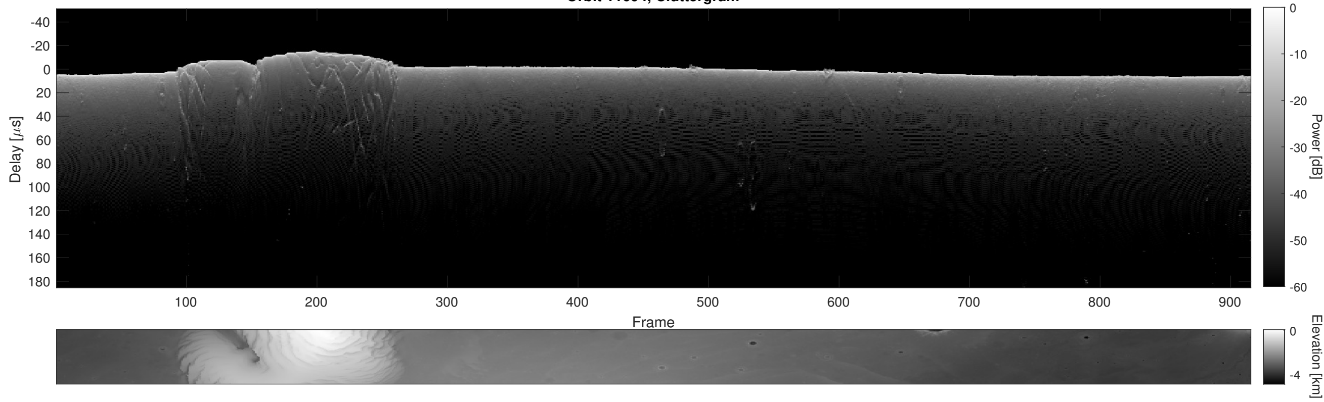
Orbit 11694, Cluttergram
