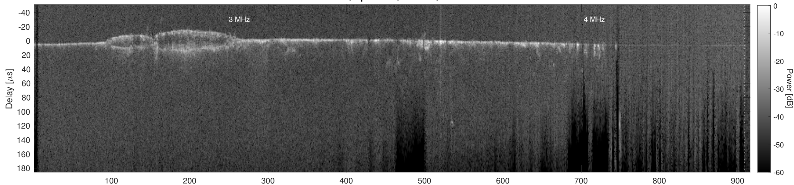
Orbit 11694, Cluttergram
