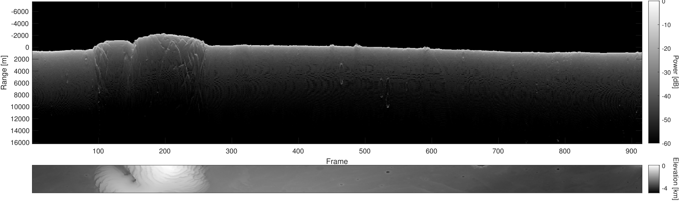
Orbit 11694, Depth-Corrected Cluttergram
