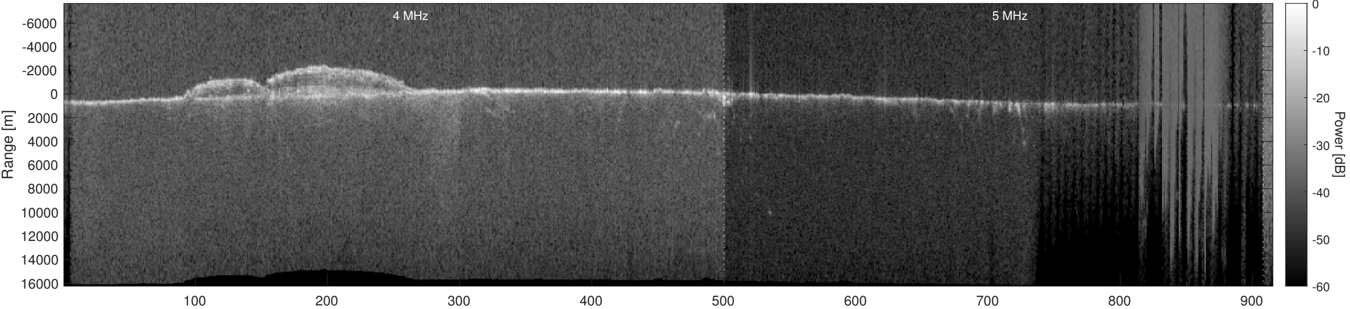
Orbit 11694, Optimized, Window, Depth-Corrected, Channel 2
