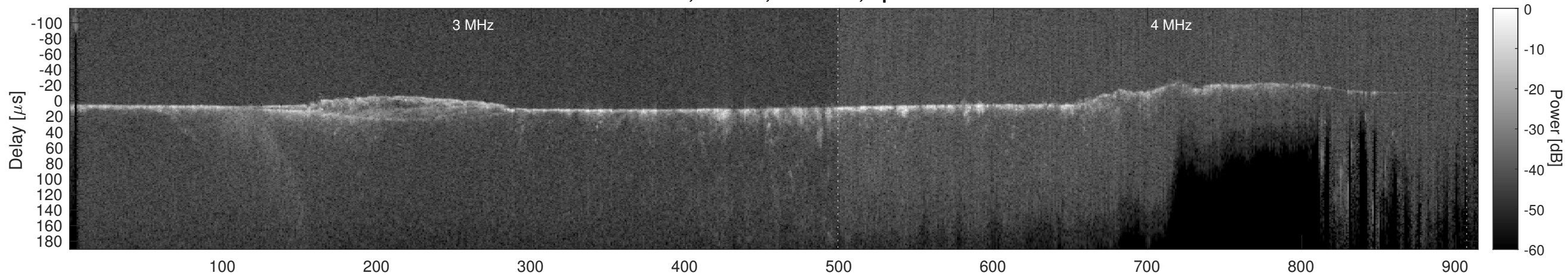
Orbit 11696, Cluttergram
