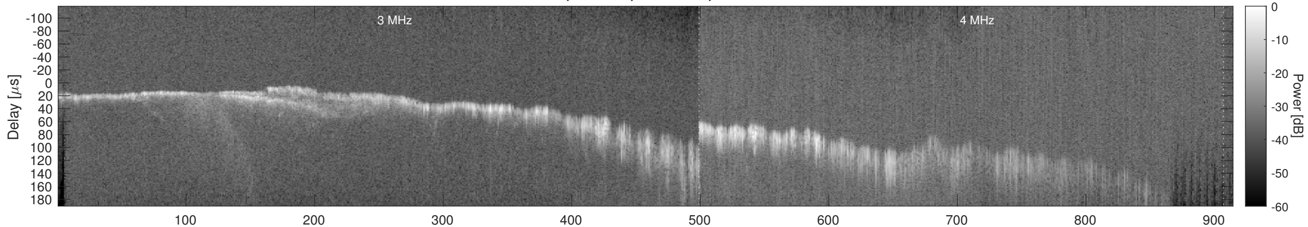
Orbit 11696, Window, Channel 2, Chapman
