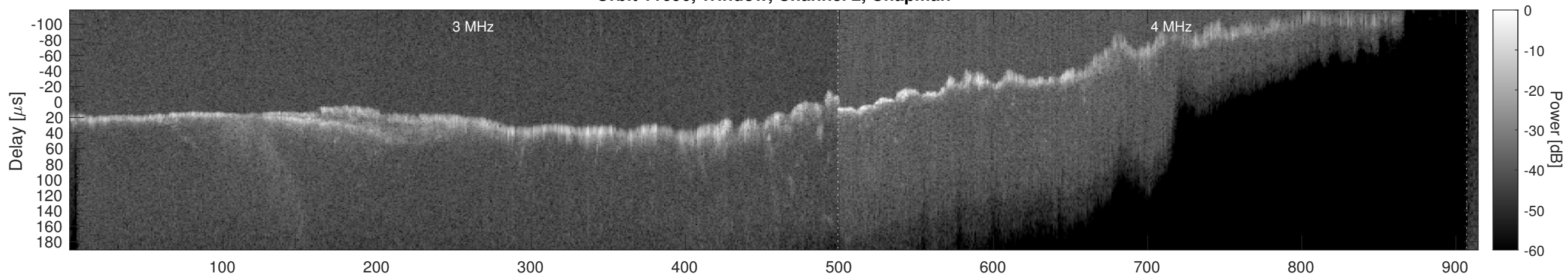
Orbit 11696, Window, Channel 2, Optimized
